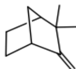
Canfeno
